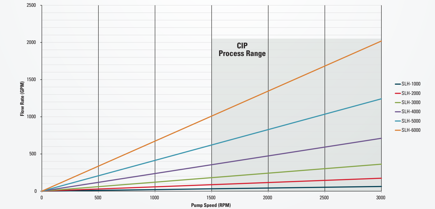
SLH Twin Screw Pump Capacity Curves
