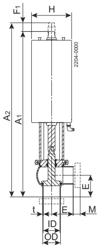
Figure 1. Shut-off valve
