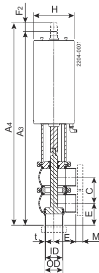
Figure 2. Change-over valve
