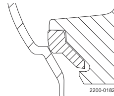
Figure 3. PTFE plug seal (TR2)
