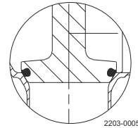
Figure 3. PTFE plug seal (TR2)
