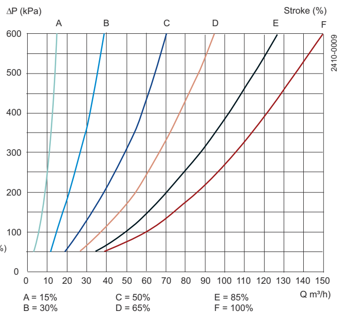
Figure 10. CPM-I-D, Kv 60
