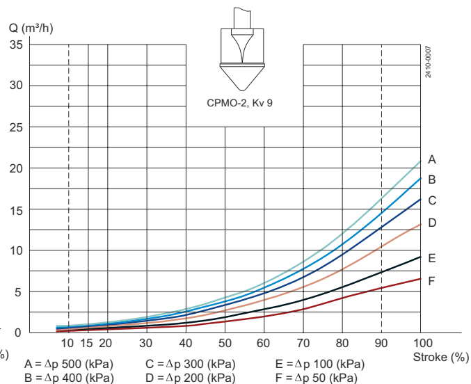
Figure 8. CPMO-2, Kv 9
