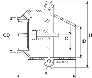
Figure 5. LKC-Drainable
