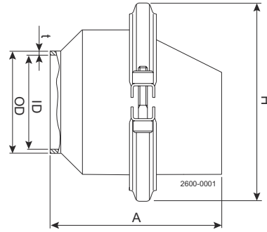
Figure 3. Horizontal mounted
