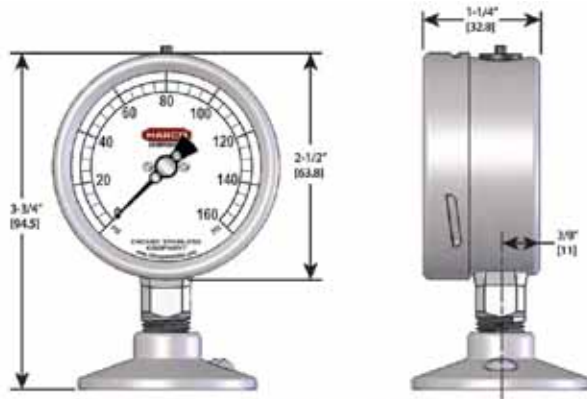
2-1/2" BOTTOM MOUNT (Shown with 1-1/2" Tri-Clamp)
