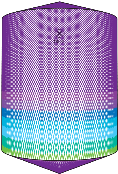
D8m H10m, Toftejorg TZ-66, 4 x ø10 mm, 0% Time = 23.3 min., Water consumption = 10868 l
