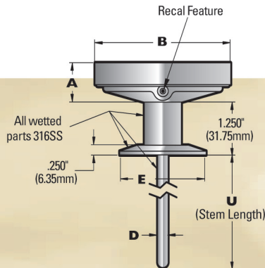
BACK MOUNT (shown with Tri-Clamp®)
