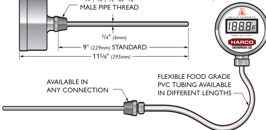
REMOTE MOUNT (shown with 1/2" NPT)
