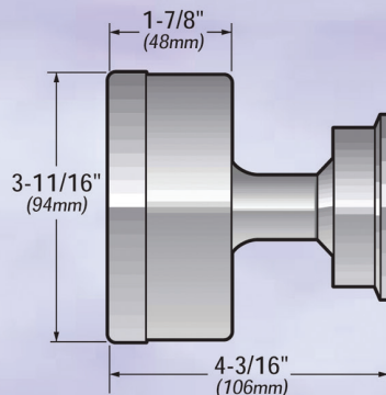
BACK MOUNT (shown with 2" Tri-Clamp®)
