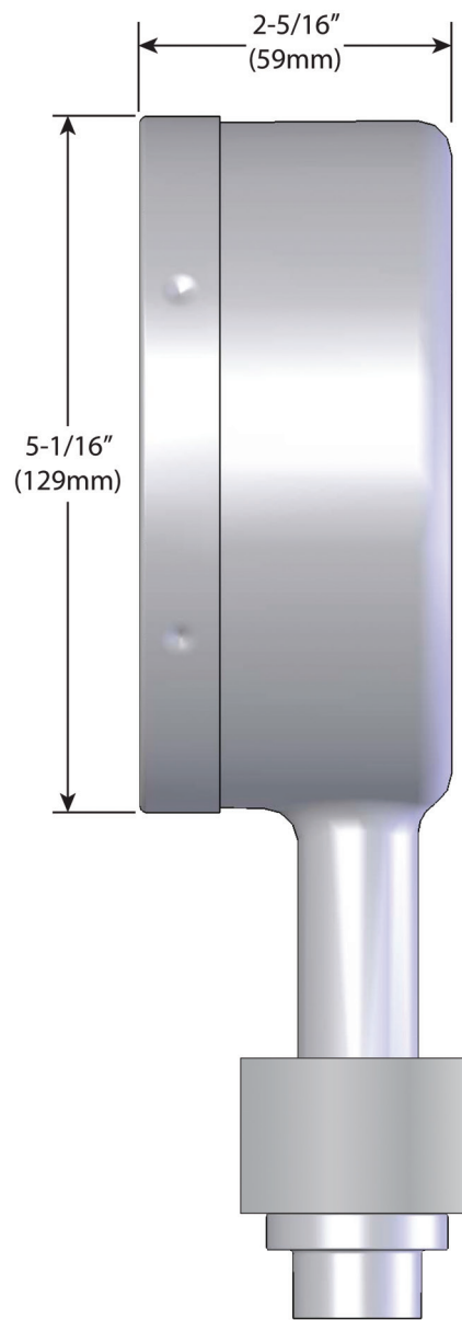
SIDE VIEW (Shown with 2 Bolt Flange)
