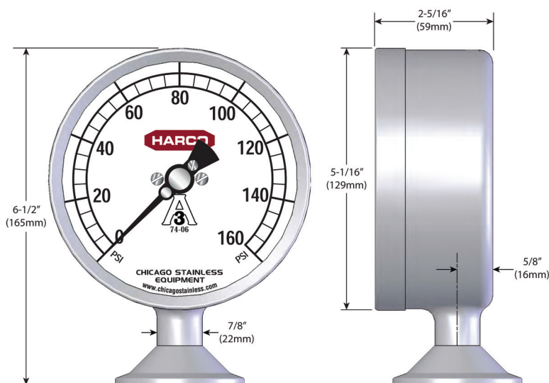
5" BOTTOM MOUNT (Shown with 2" Tri-Clamp)
