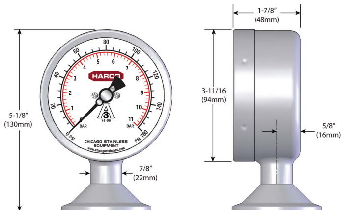
3-1/2" BOTTOM MOUNT (Shown with 2" Tri-Clamp)
