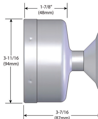
3-1/2" BACK MOUNT (Shown with 2" Tri-Clamp)
