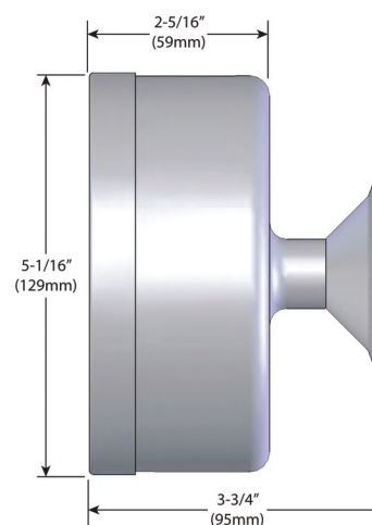
5" BACK MOUNT (Shown with 2" Tri-Clamp)
